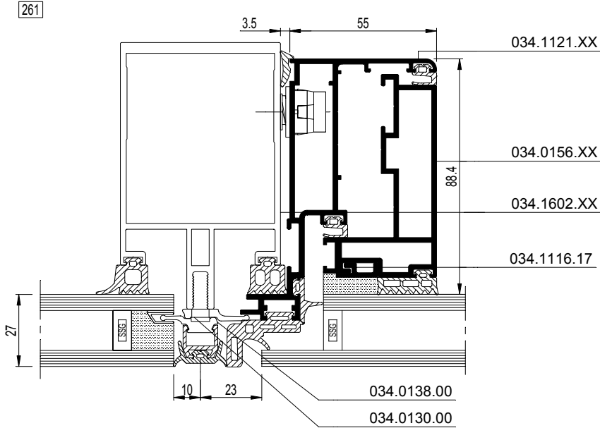
CW60-261003.dxf CW60-261003.dwg
