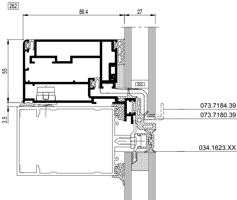
CW60-262003.dxf CW60-262003.dwg
