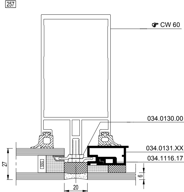
CW60-257001.dxf CW60-257001.dwg
