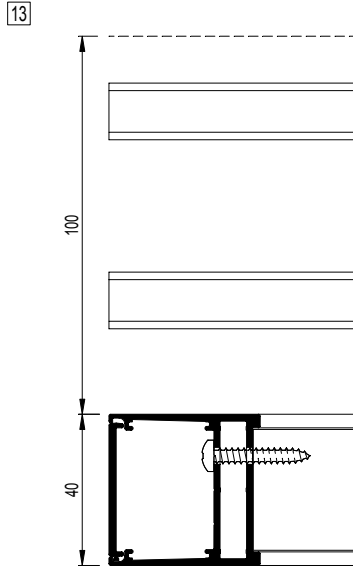
BS40-013001.dxf BS40-013001.dwg
